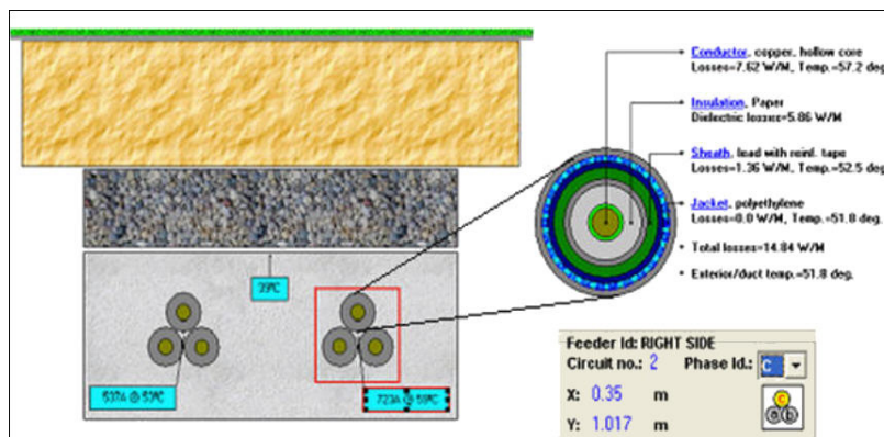
CYMCAP Model and results for a multi-layer installation
